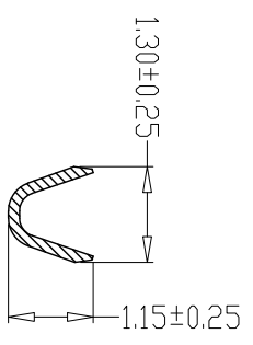
SEC. B-B
